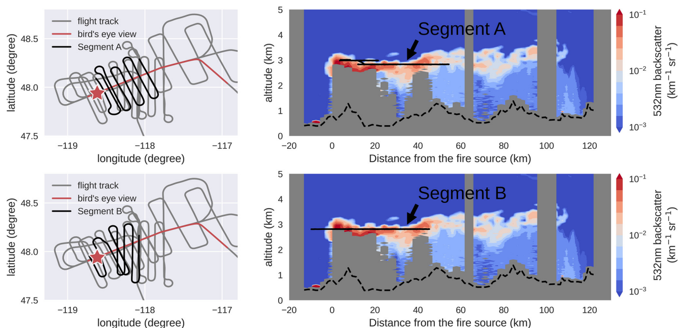
Figure 1. (Left) Flight tracks and (right) 532 nm backscatter ratio measured using National Aeronautics and Space Administration (NASA) Differential Absorption Lidar (DIAL). Red stars in the left panel represents the approximate location of the fire source. Gray lines in the left panel shows the entire flight track, while the red lines denote the flight legs when the aircraft was flying above the smoke, producing the “bird’s eye view” that are shown on the right panel. The flight altitudes during Segments A and B (solid black lines in the right panel) are overlaid on top of the “bird’s eye view” curtain in the right panel, but Segments A and B occurred at different times than the “bird’s eye view” flight.
