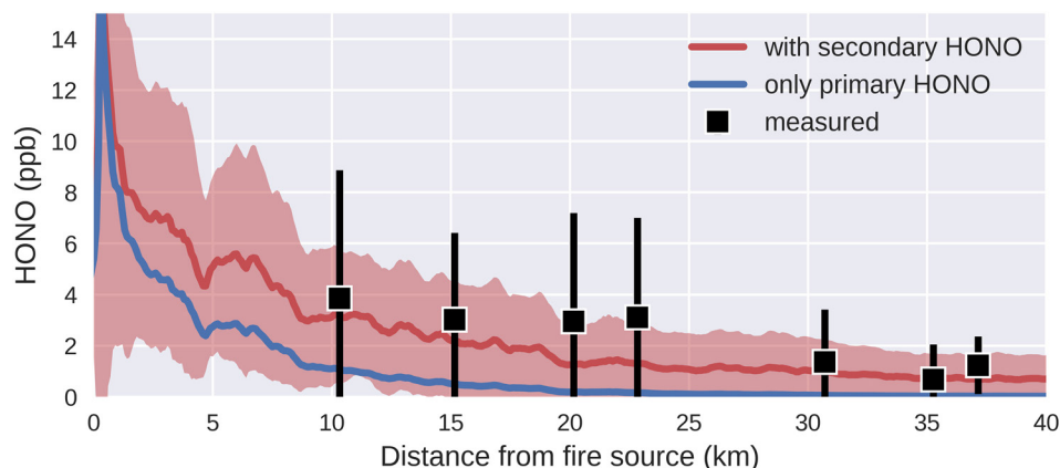
Figure 11. Measured plume-wide averages of HONO compared to modeled in different model scenarios: with both primary and secondary HONO (dark red, same as that in Figure 3), with only primary HONO and no secondary HONO production (blue).
